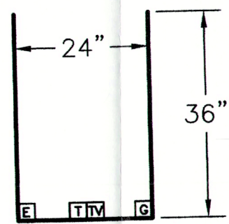
SECONDARY TRENCH STREET CROSSING
